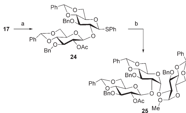
Scheme 3. Iterative preparation of α,β-triglucoside 25 . a) 1-Benzenesulfonyl piperidine (1 equiv), Tf 2 O (1.1 equiv), 2,4,6-tri-tert-butylpyrimidine (2 equiv), MS 4 Å, CH 2 Cl 2 , -60 °C, 15 min, then 10 (1.25 equiv) 1 h, 70%. b) The same conditions as in (a) but with 3 (1.25 equiv), 66% (81% based on recovered donor 24 ).
